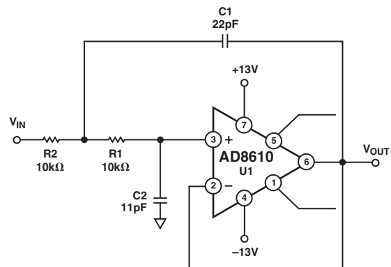
Figure 29. Second-Order Low-Pass Filter
