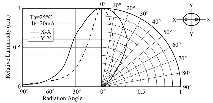
■ Directivity (NSPB636AS)
