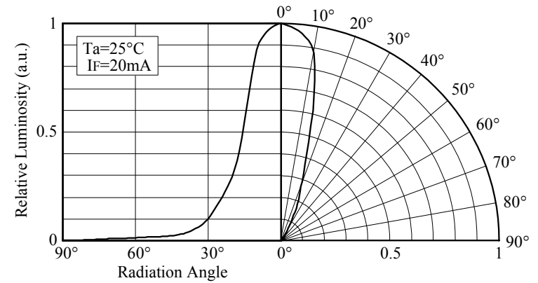
■ Directivity (NSPG510(S))
